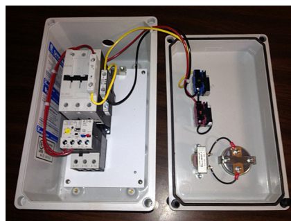
Small enclosure or Starter Boxes
