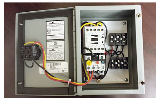
Small enclosure or Starter Boxes
