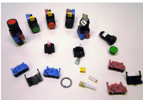
Oil Tight 30mm & 22mm Switch Assembly
